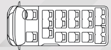
18 Seat Layout
