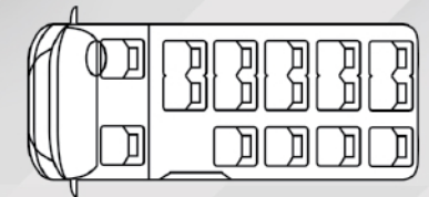
16 Seat Layout
